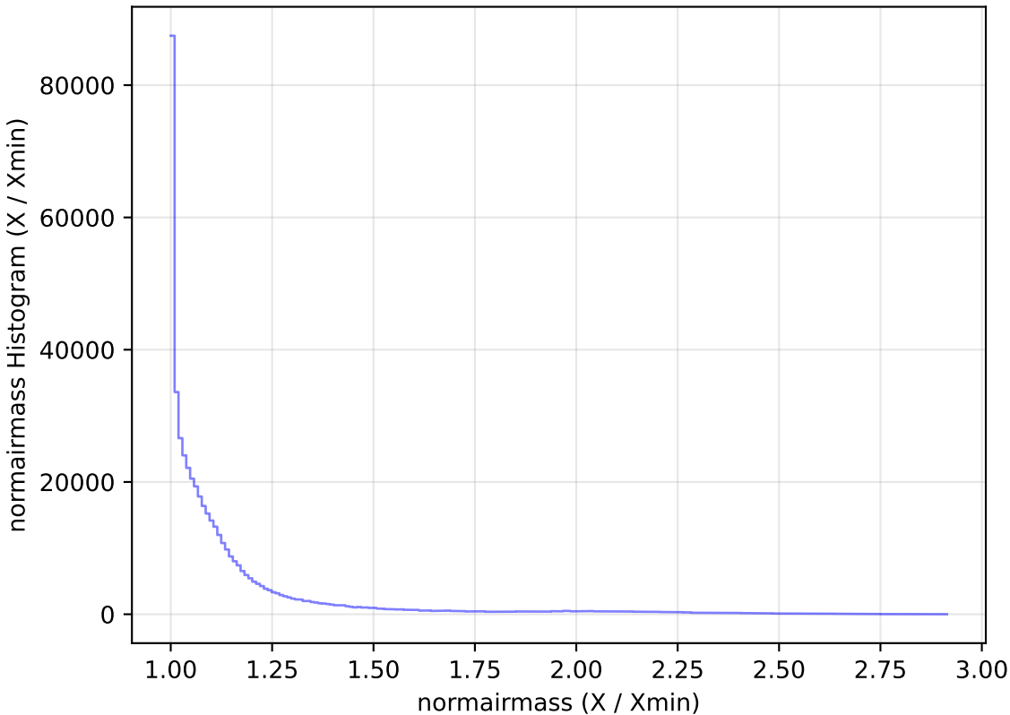
roll_pause_mjdp60_v3.4_10yrs WFD i band: normairmass Histogram
