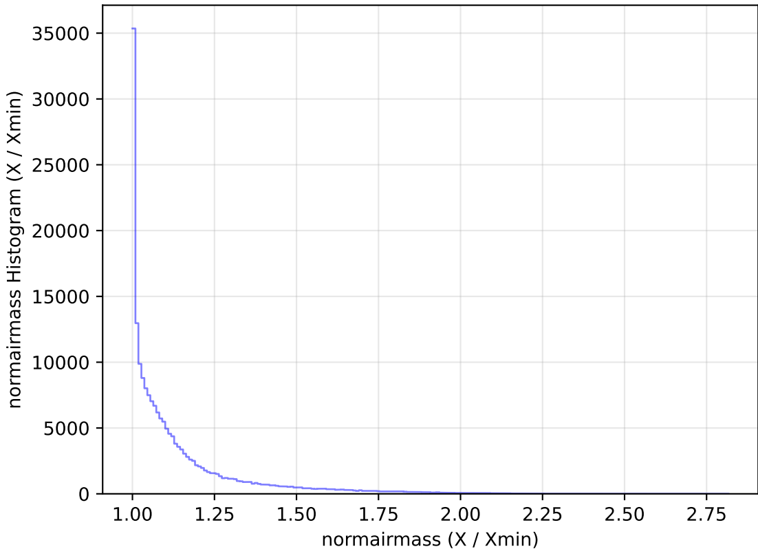
roll_pause_mjdp60_v3.4_10yrs WFD g band: normairmass Histogram
