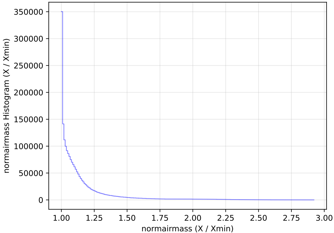
roll_pause_mjdp60_v3.4_10yrs WFD all bands: normairmass Histogram
