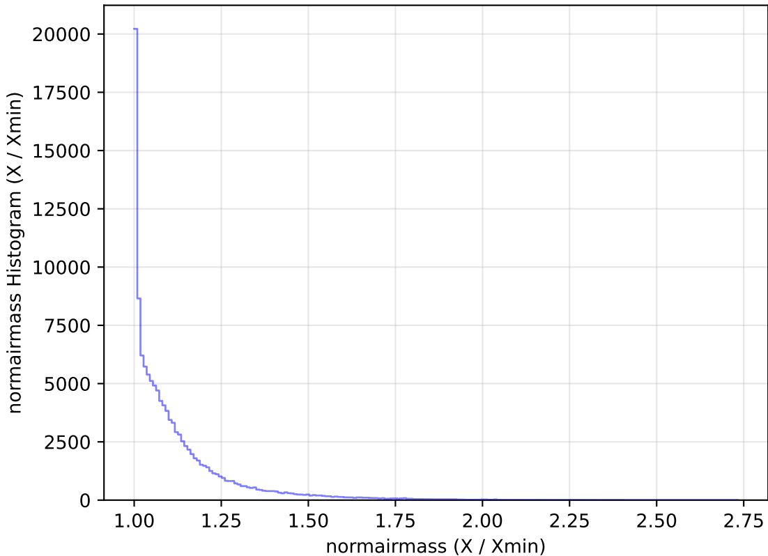
roll_pause_mjdp60_v3.4_10yrs All sky u band: normairmass Histogram
