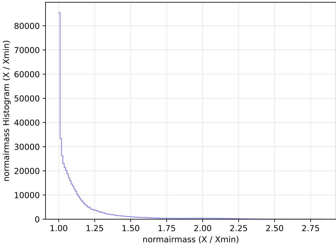
roll_pause_mjdp60_v3.4_10yrs All sky r band: normairmass Histogram
