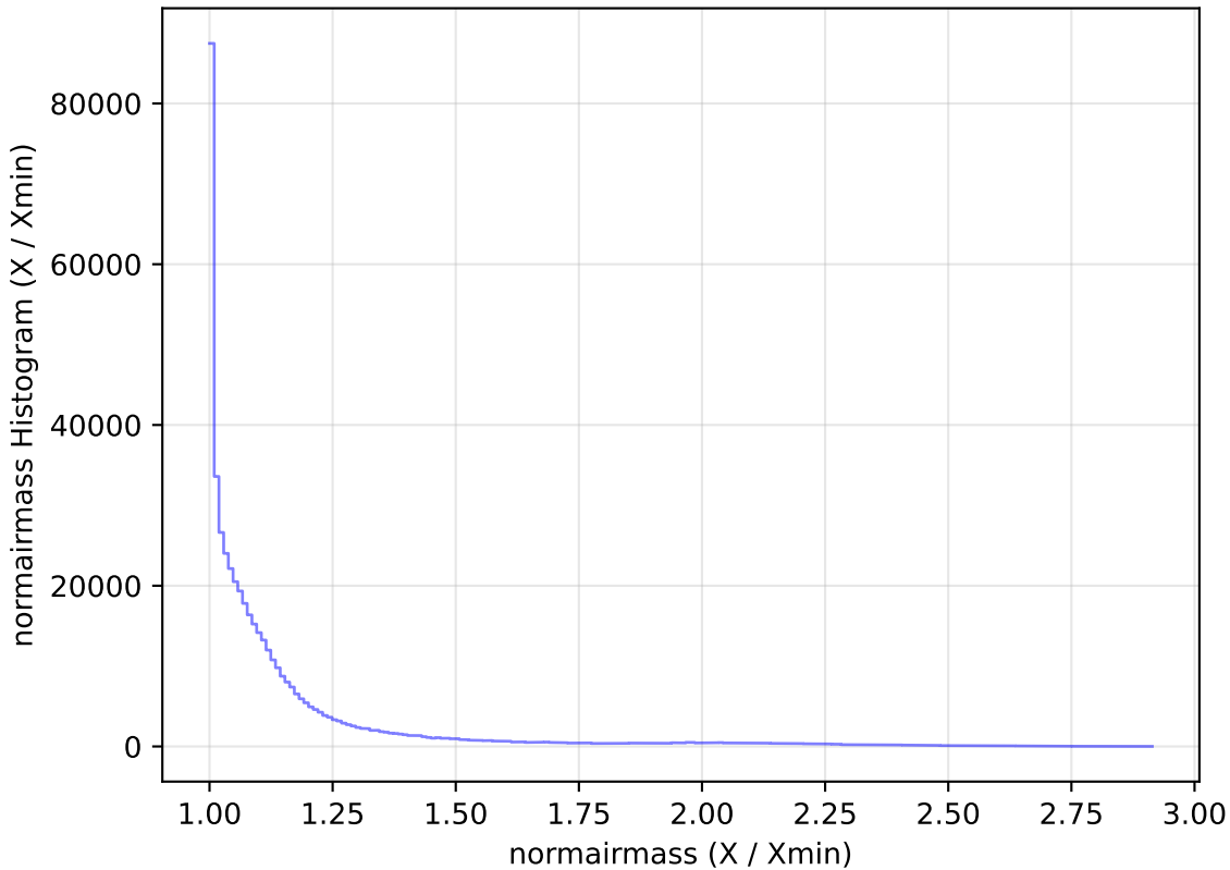
roll_pause_mjdp60_v3.4_10yrs All sky i band: normairmass Histogram
