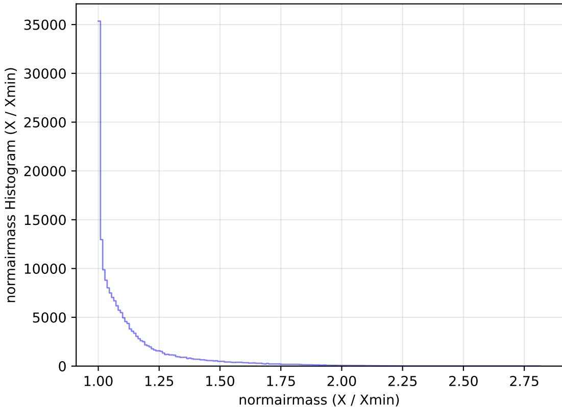
roll_pause_mjdp60_v3.4_10yrs All sky g band: normairmass Histogram
