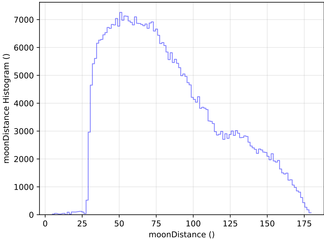
roll_pause_mjdp60_v3.4_10yrs WFD z band: moonDistance Histogram
