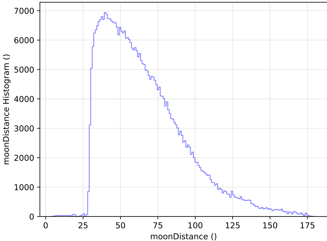
roll_pause_mjdp60_v3.4_10yrs WFD y band: moonDistance Histogram
