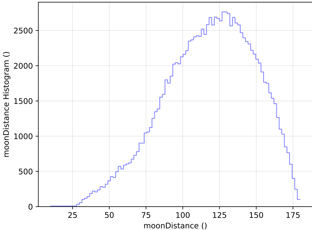
roll_pause_mjdp60_v3.4_10yrs WFD u band: moonDistance Histogram
