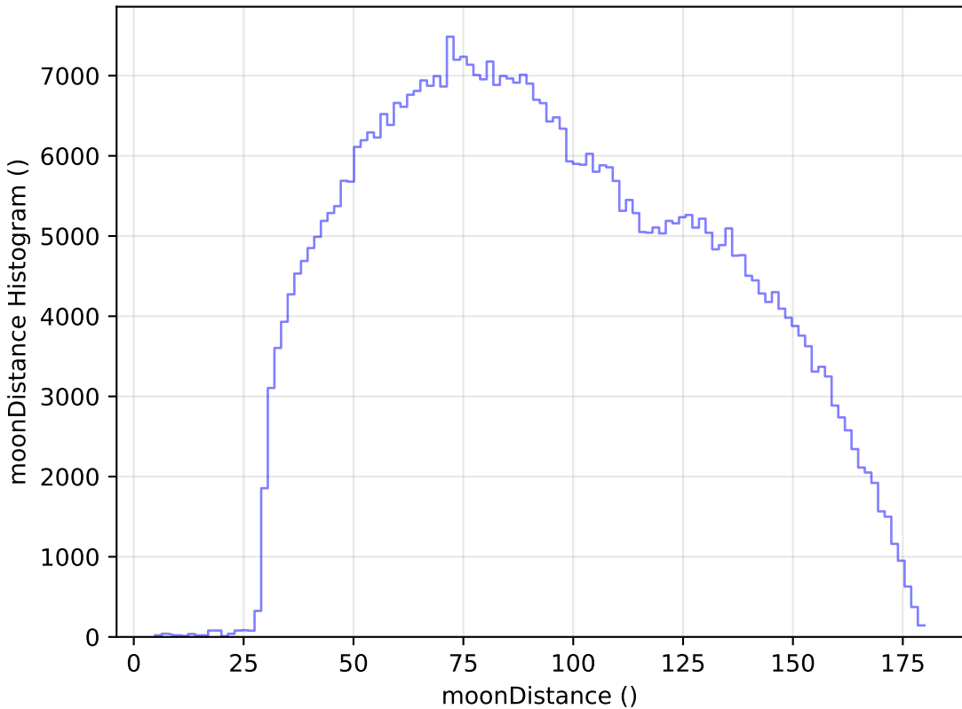
roll_pause_mjdp60_v3.4_10yrs WFD i band: moonDistance Histogram
