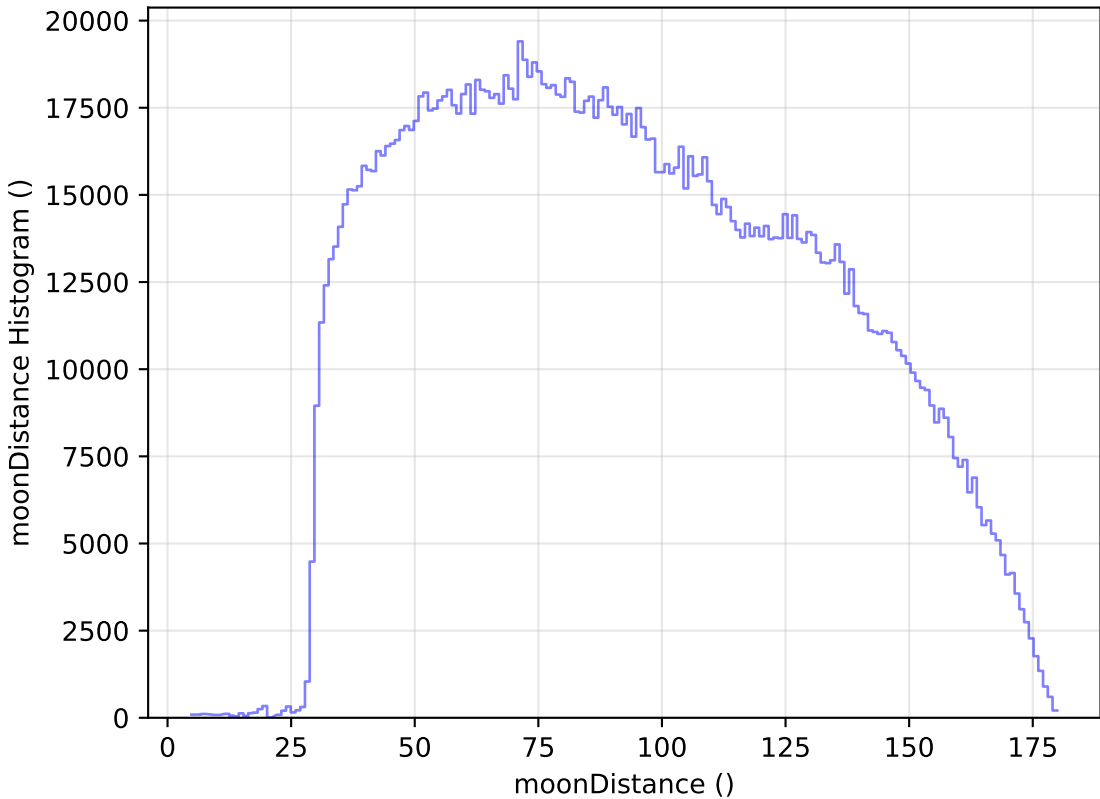
roll_pause_mjdp60_v3.4_10yrs WFD all bands: moonDistance Histogram
