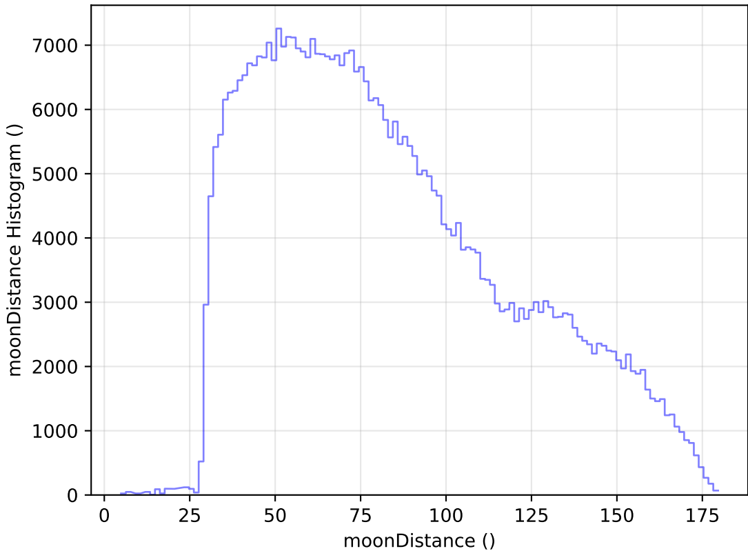
roll_pause_mjdp60_v3.4_10yrs All sky z band: moonDistance Histogram
