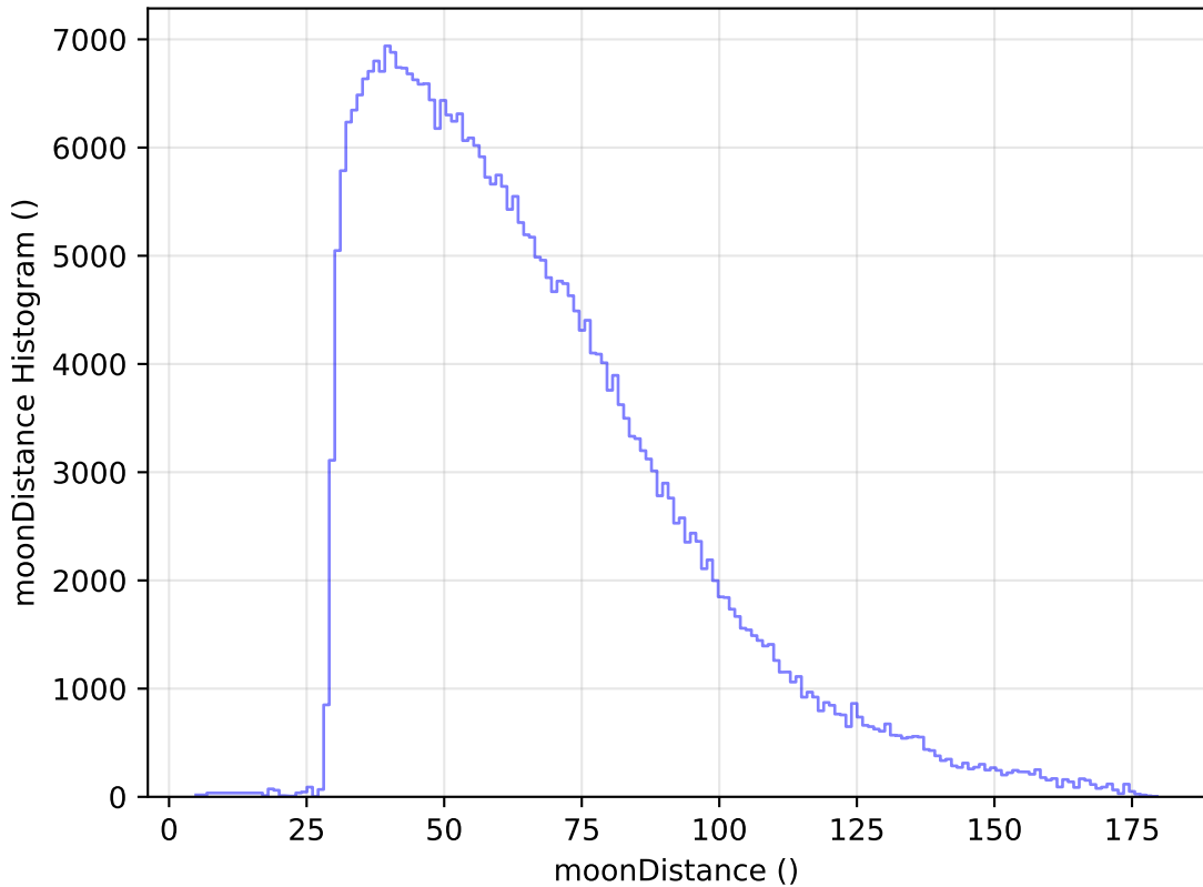
roll_pause_mjdp60_v3.4_10yrs All sky y band: moonDistance Histogram
