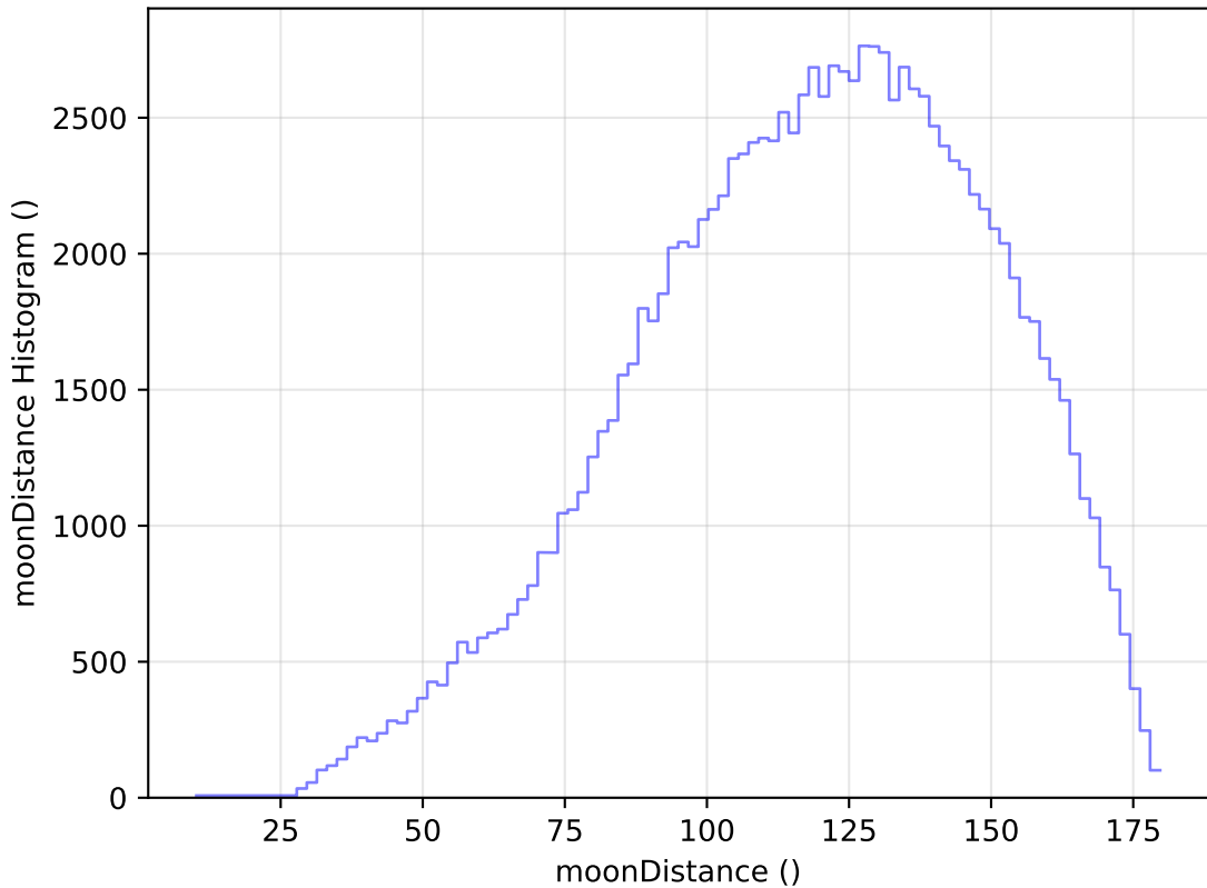
roll_pause_mjdp60_v3.4_10yrs All sky u band: moonDistance Histogram
