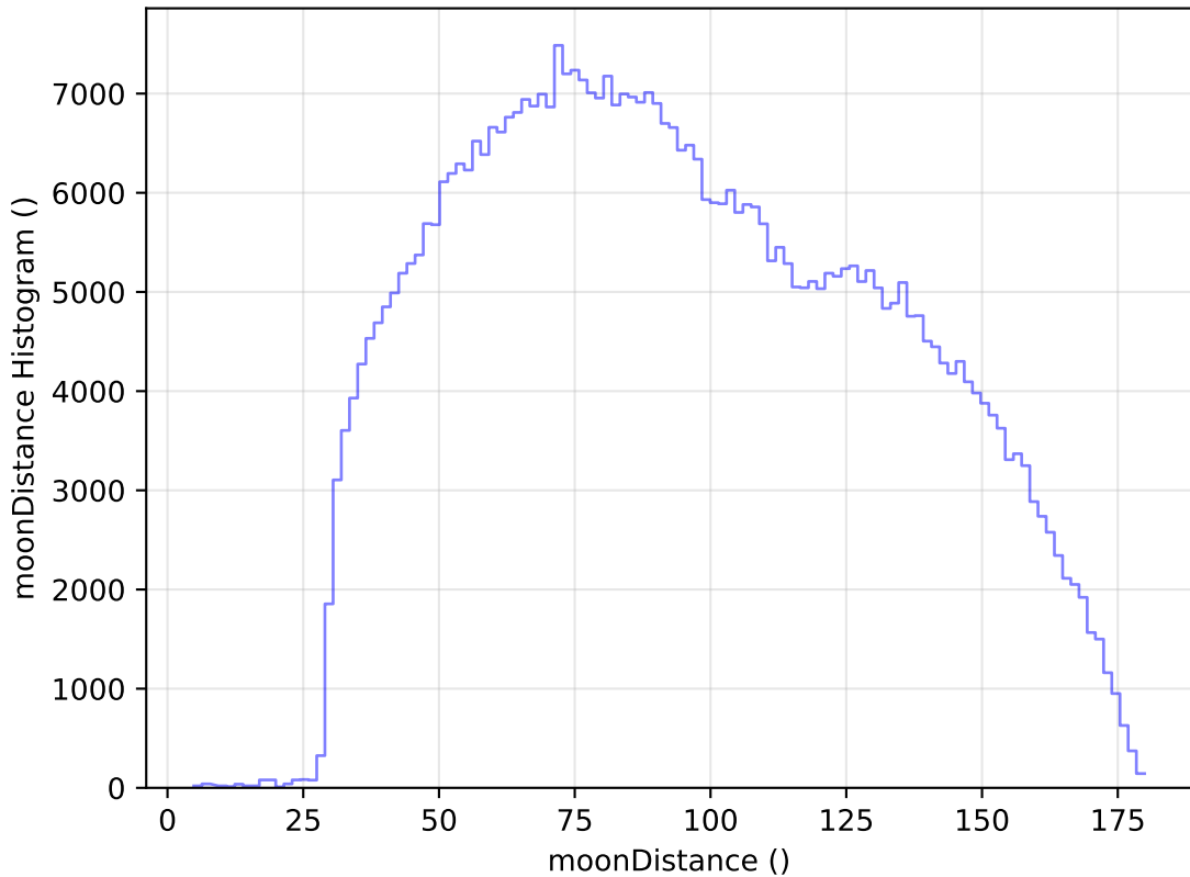
roll_pause_mjdp60_v3.4_10yrs All sky i band: moonDistance Histogram
