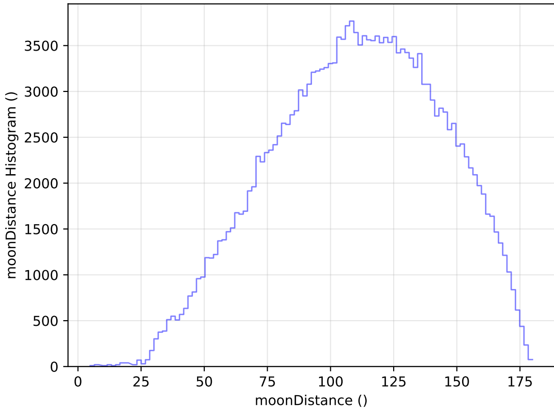
roll_pause_mjdp60_v3.4_10yrs All sky g band: moonDistance Histogram
