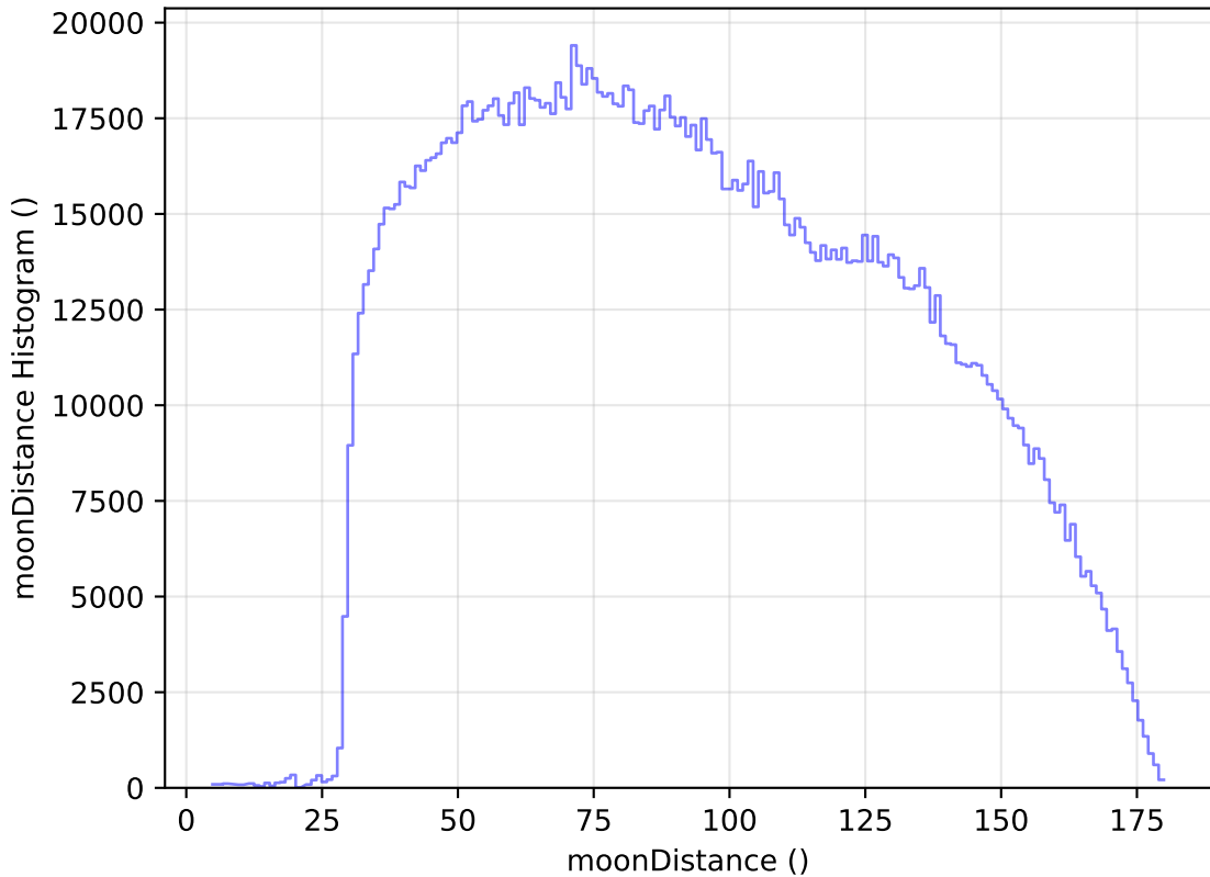
roll_pause_mjdp60_v3.4_10yrs All sky all bands: moonDistance Histogram
