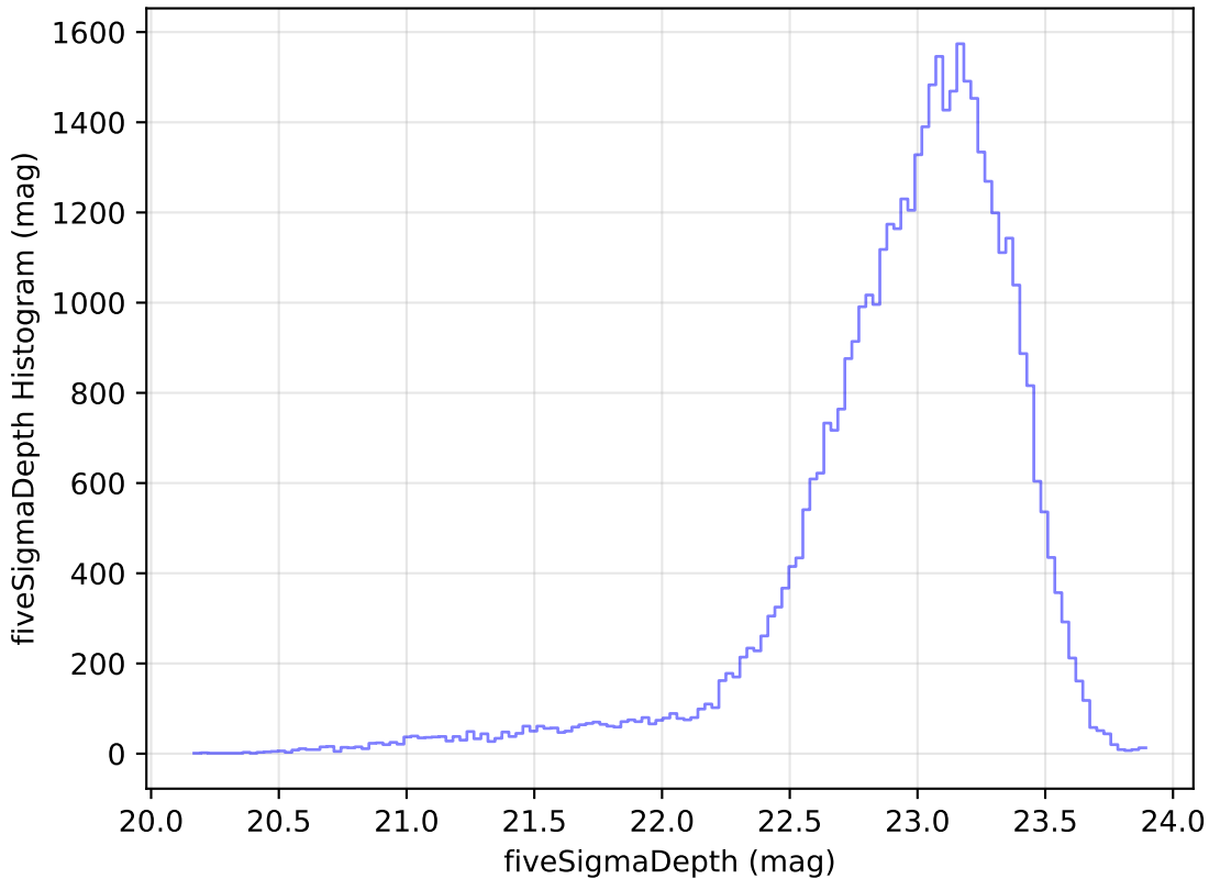
roll_pause_mjdp60_v3.4_10yrs Yr 1 z band: fiveSigmaDepth Histogram
