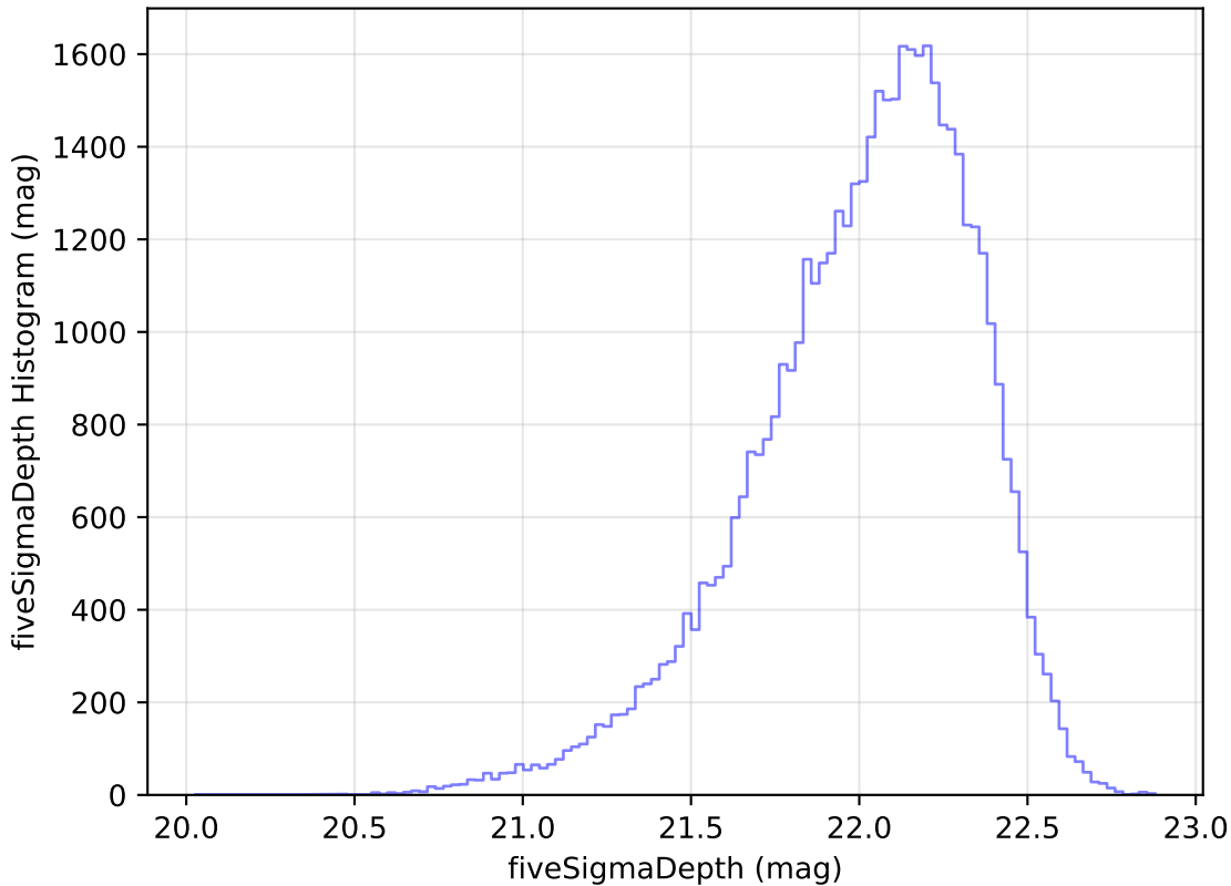
roll_pause_mjdp60_v3.4_10yrs Yr 1 y band: fiveSigmaDepth Histogram
