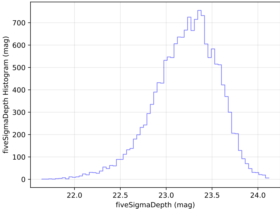
roll_pause_mjdp60_v3.4_10yrs Yr 1 u band: fiveSigmaDepth Histogram
