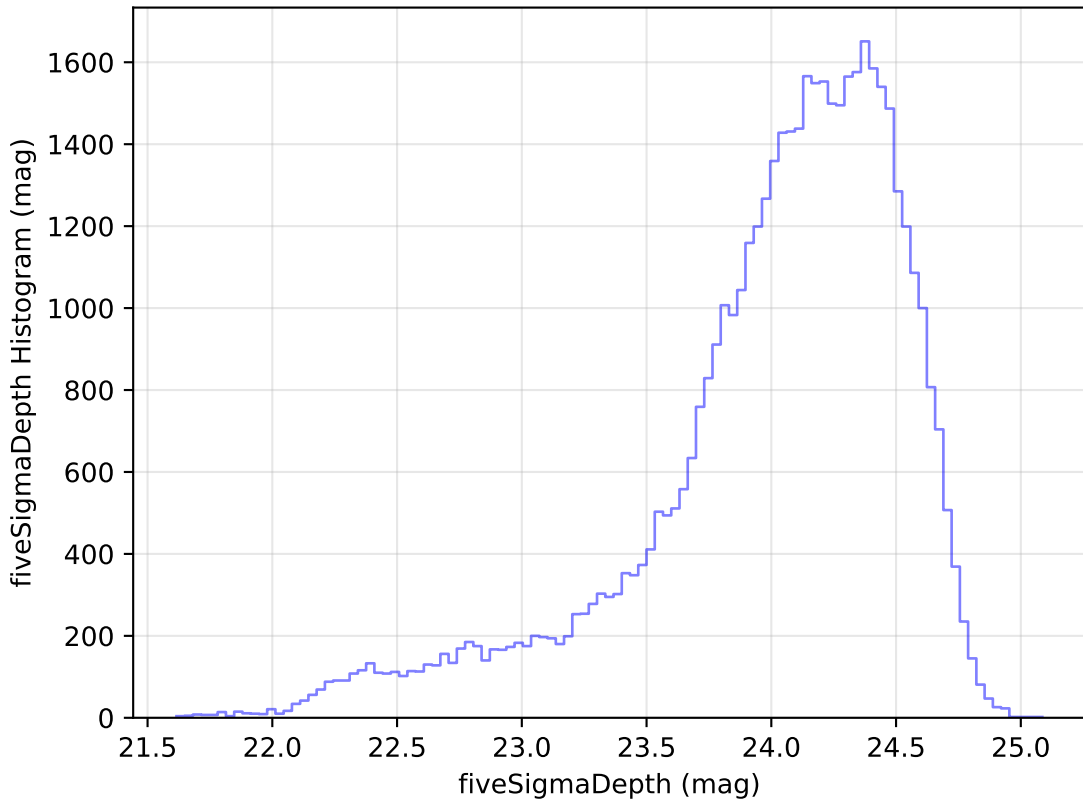
roll_pause_mjdp60_v3.4_10yrs Yr 1 r band: fiveSigmaDepth Histogram
