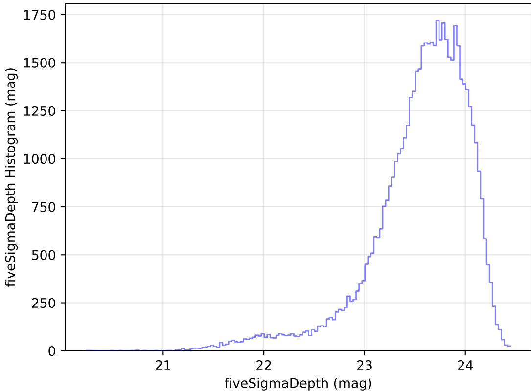
roll_pause_mjdp60_v3.4_10yrs Yr 1 i band: fiveSigmaDepth Histogram
