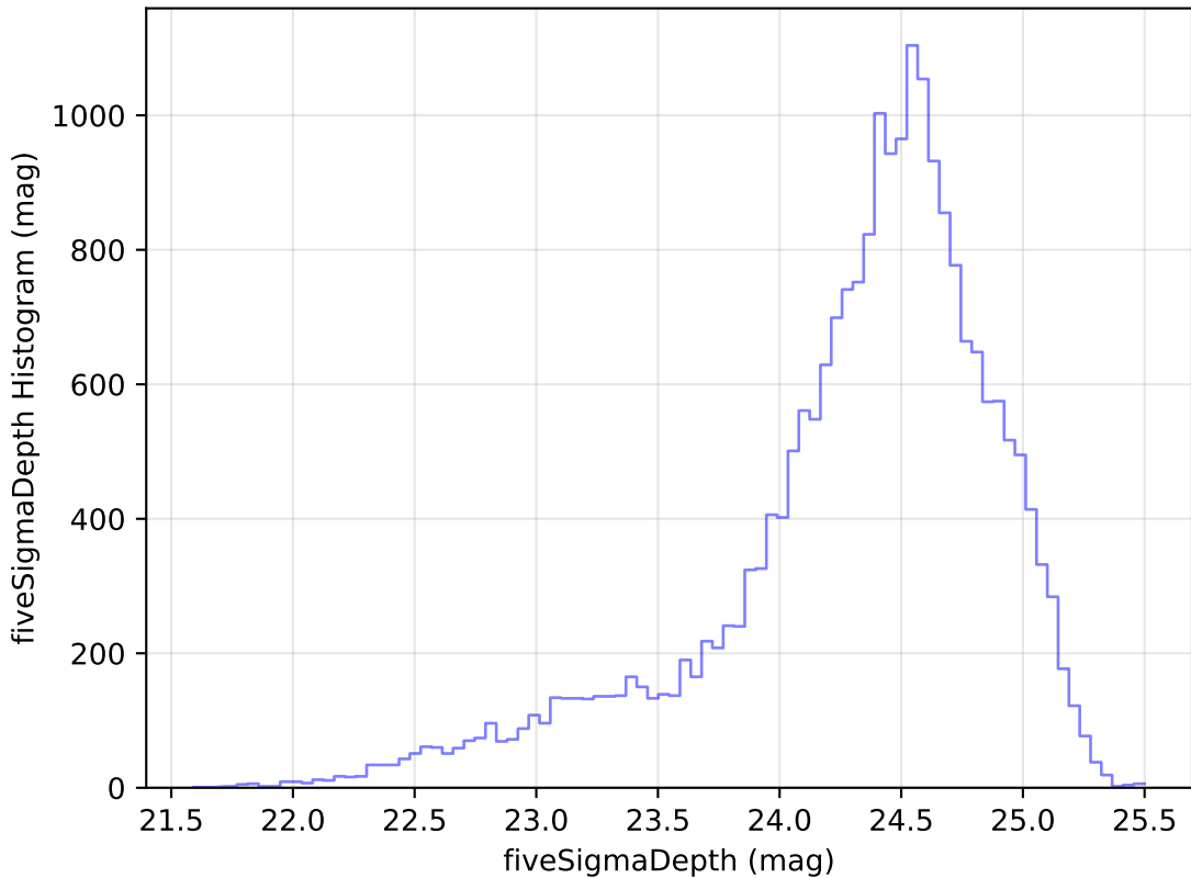
roll_pause_mjdp60_v3.4_10yrs Yr 1 g band: fiveSigmaDepth Histogram
