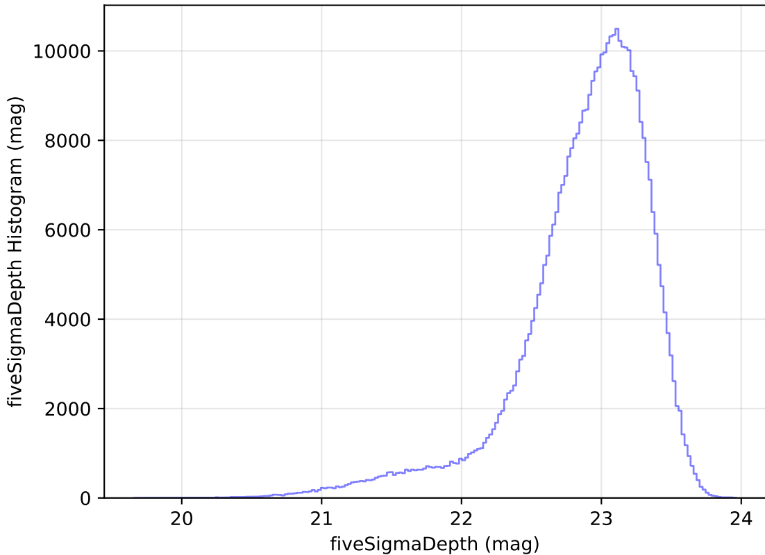
roll_pause_mjdp60_v3.4_10yrs WFD z band: fiveSigmaDepth Histogram
