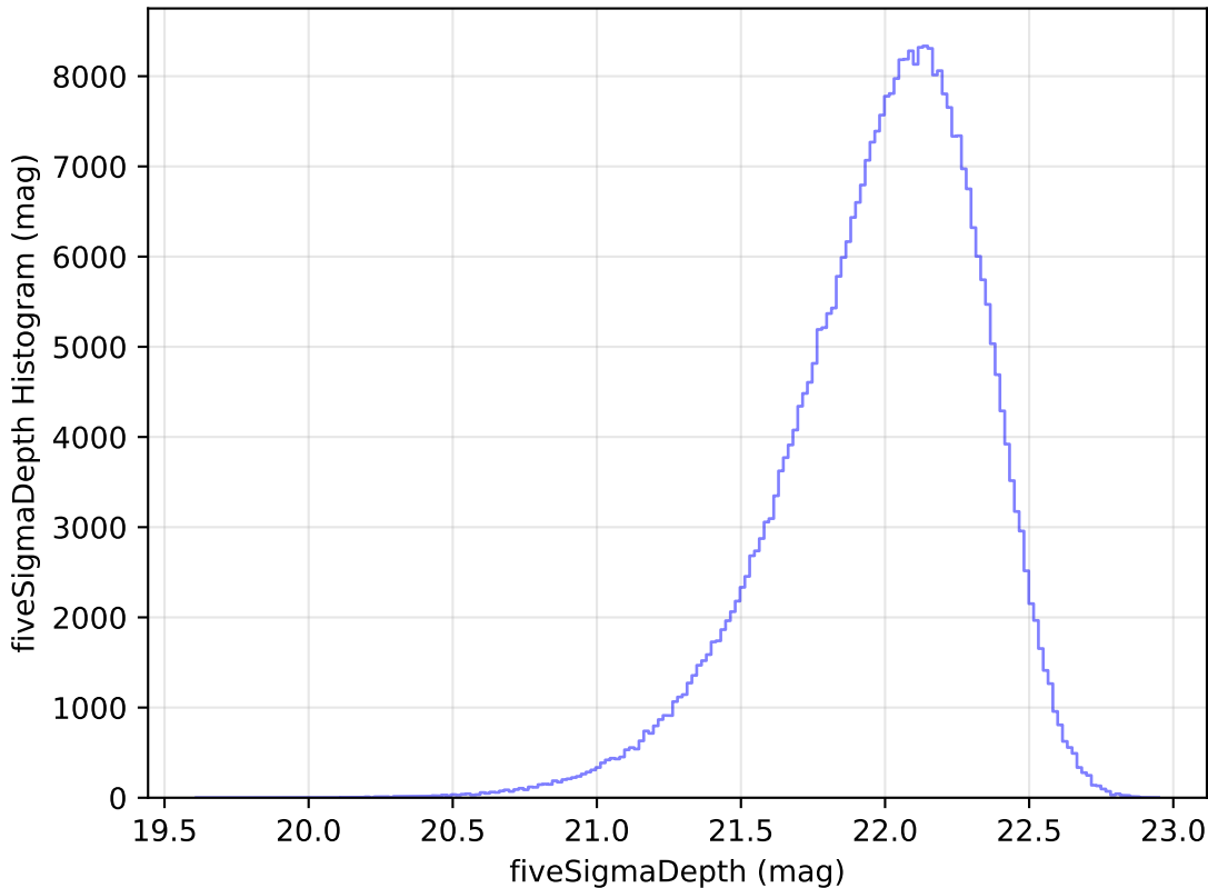
roll_pause_mjdp60_v3.4_10yrs WFD y band: fiveSigmaDepth Histogram
