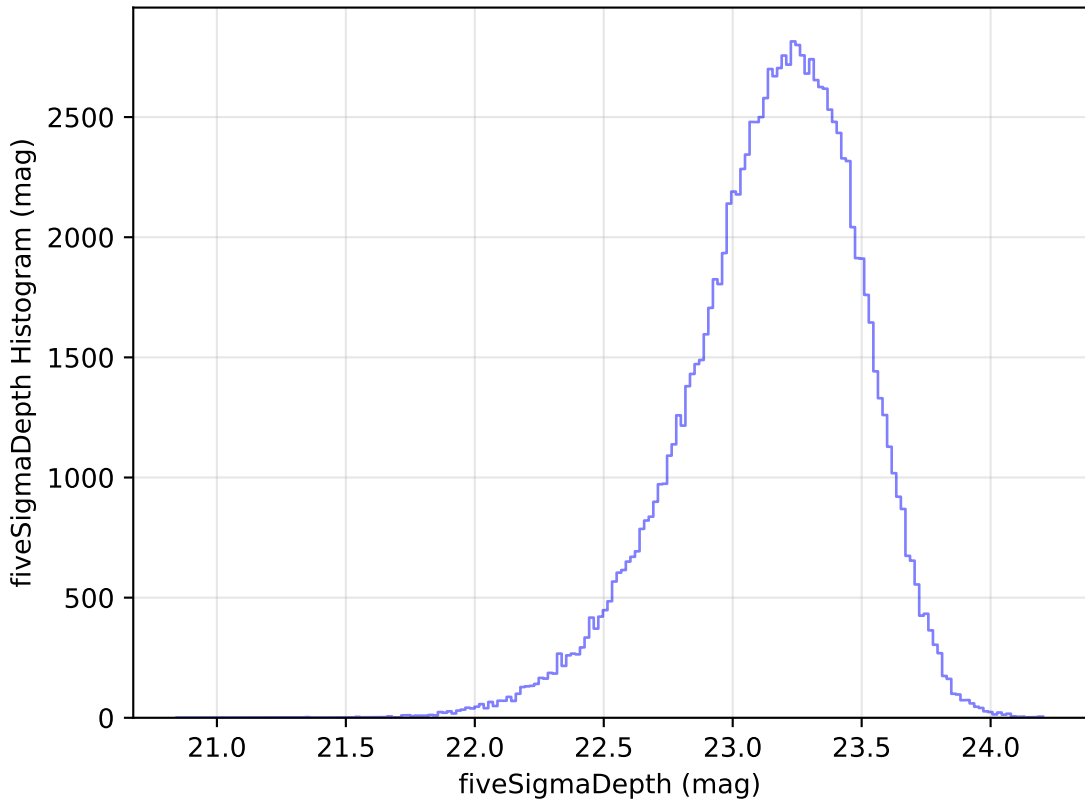
roll_pause_mjdp60_v3.4_10yrs WFD u band: fiveSigmaDepth Histogram
