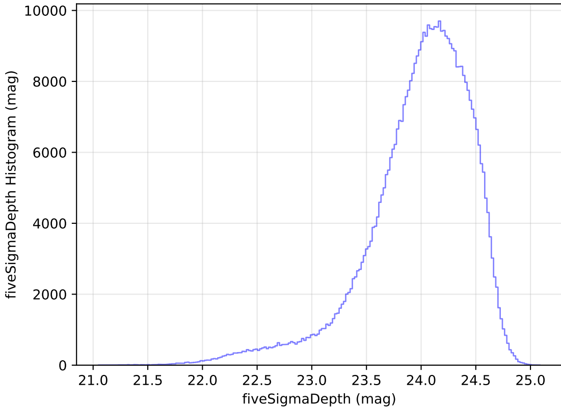
roll_pause_mjdp60_v3.4_10yrs WFD r band: fiveSigmaDepth Histogram
