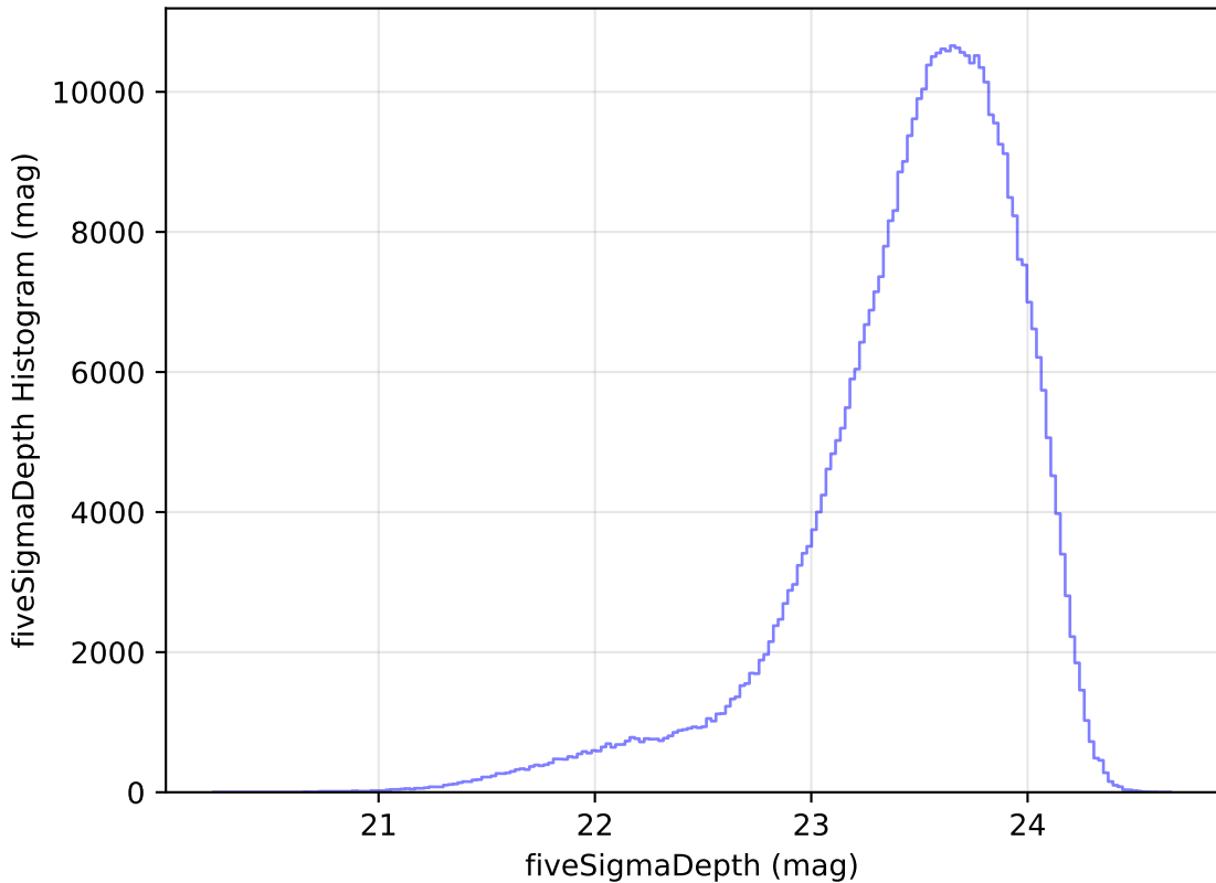
roll_pause_mjdp60_v3.4_10yrs WFD i band: fiveSigmaDepth Histogram
