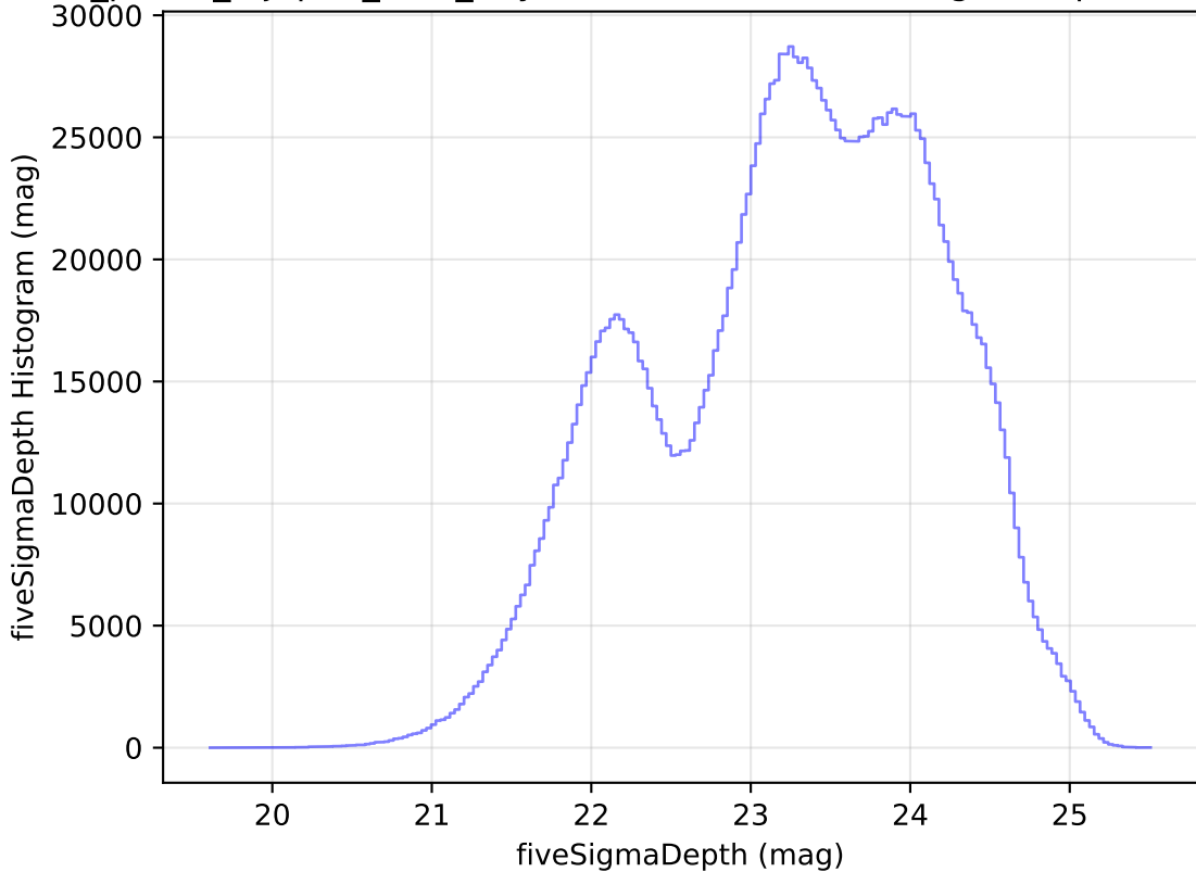
roll_pause_mjdp60_v3.4_10yrs WFD all bands: fiveSigmaDepth Histogram
