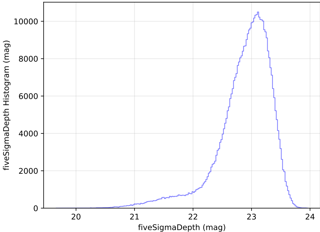
roll_pause_mjdp60_v3.4_10yrs All sky z band: fiveSigmaDepth Histogram
