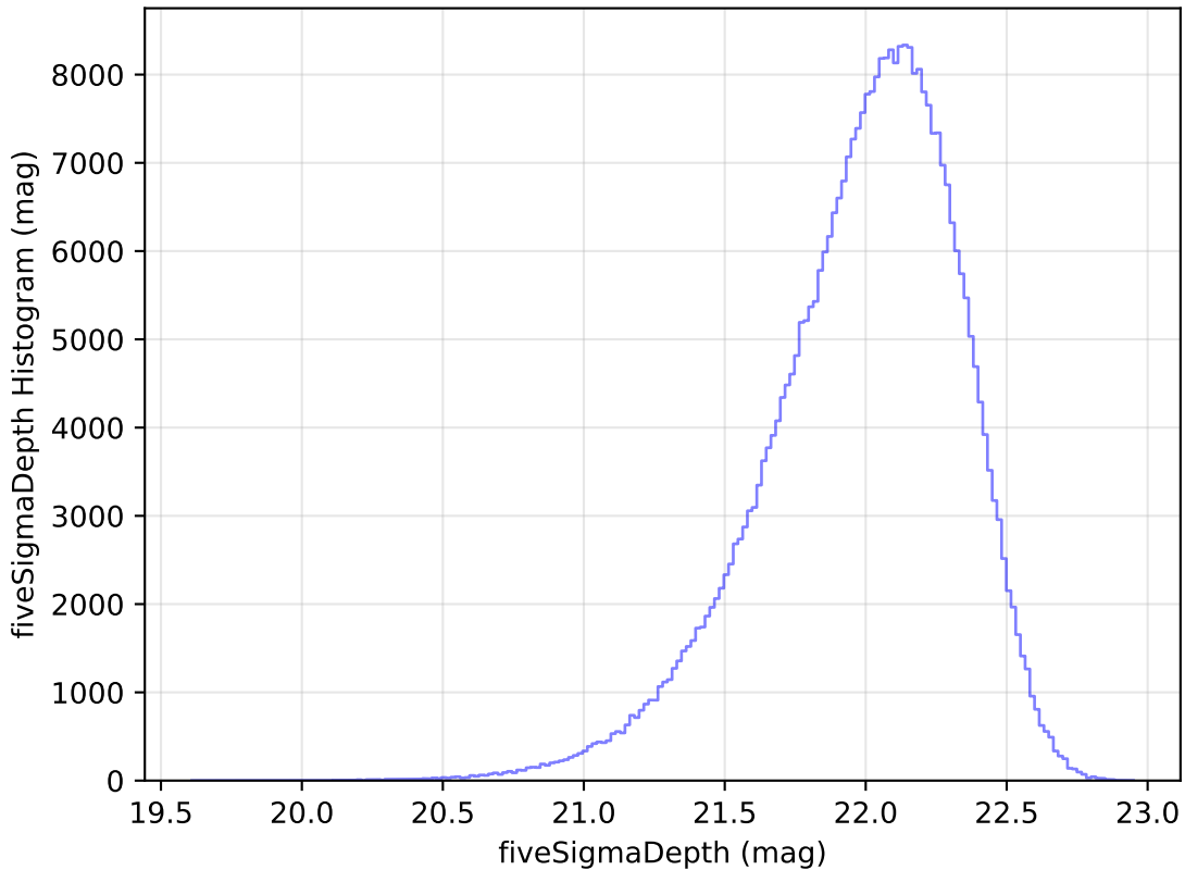
roll_pause_mjdp60_v3.4_10yrs All sky y band: fiveSigmaDepth Histogram
