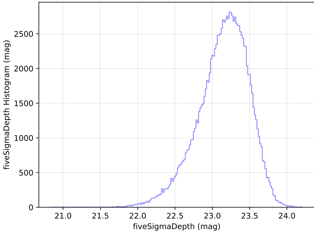
roll_pause_mjdp60_v3.4_10yrs All sky u band: fiveSigmaDepth Histogram
