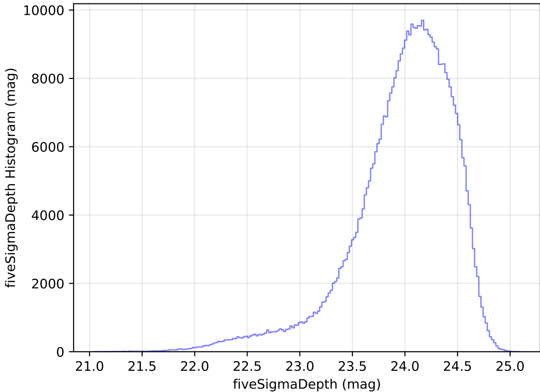
roll_pause_mjdp60_v3.4_10yrs All sky r band: fiveSigmaDepth Histogram
