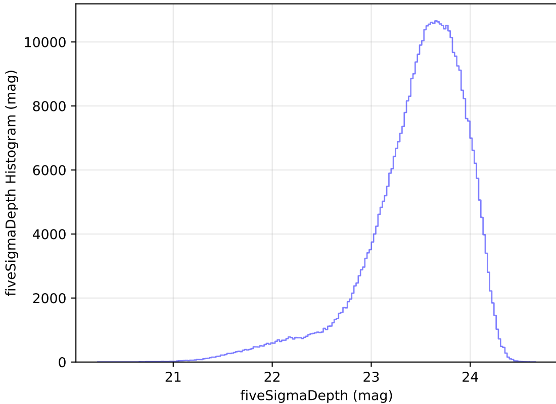
roll_pause_mjdp60_v3.4_10yrs All sky i band: fiveSigmaDepth Histogram
