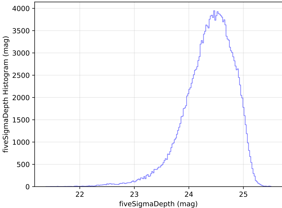
roll_pause_mjdp60_v3.4_10yrs All sky g band: fiveSigmaDepth Histogram
