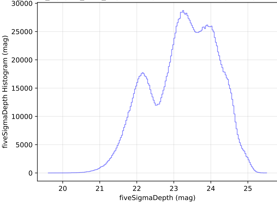
roll_pause_mjdp60_v3.4_10yrs All sky all bands: fiveSigmaDepth Histogram
