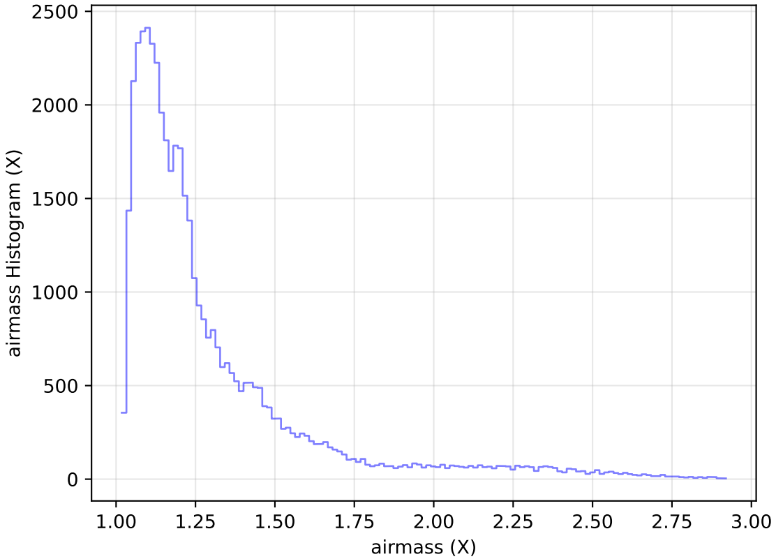
roll_pause_mjdp60_v3.4_10yrs Yr 1 z band: airmass Histogram
