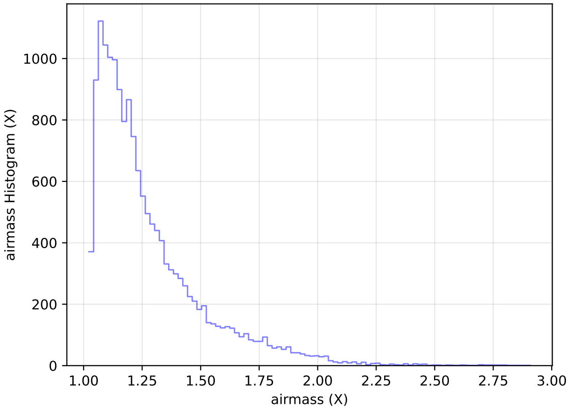
roll_pause_mjdp60_v3.4_10yrs Yr 1 u band: airmass Histogram
