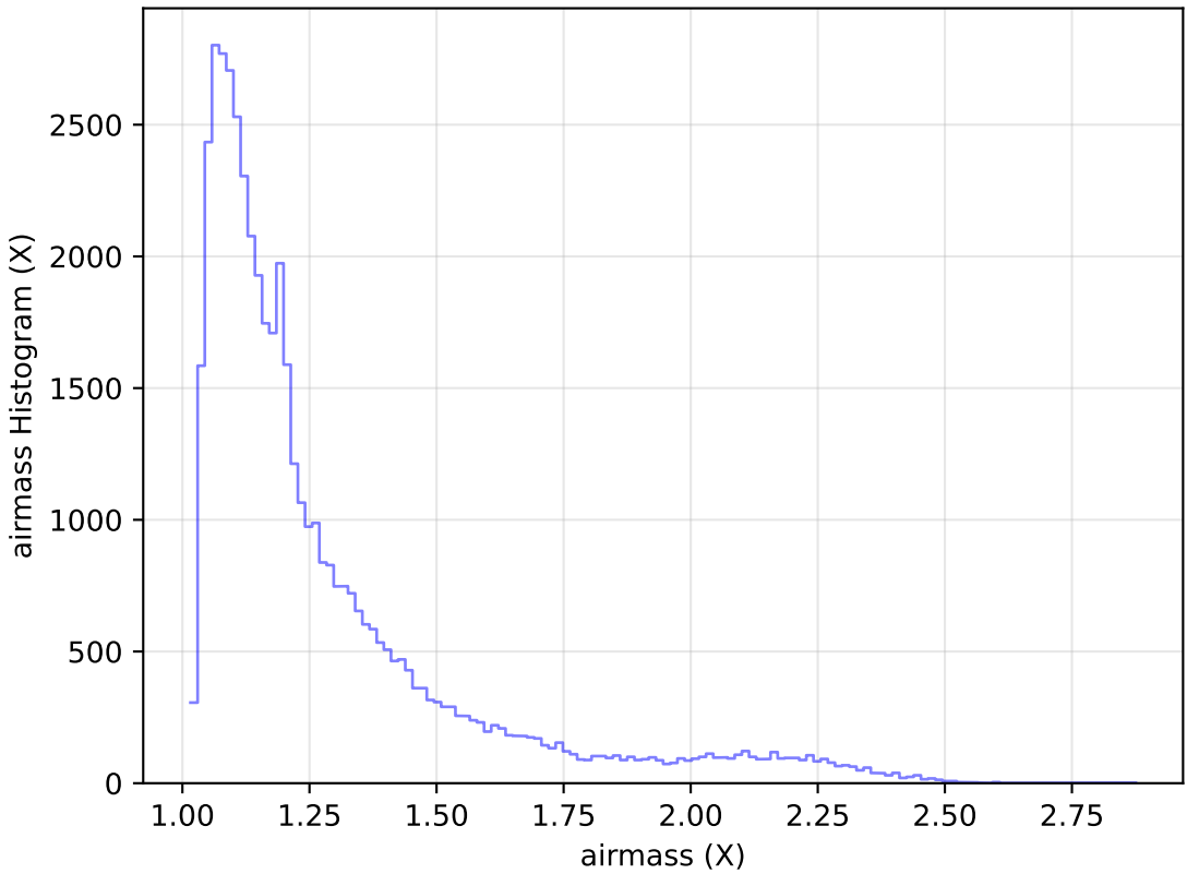
roll_pause_mjdp60_v3.4_10yrs Yr 1 r band: airmass Histogram
