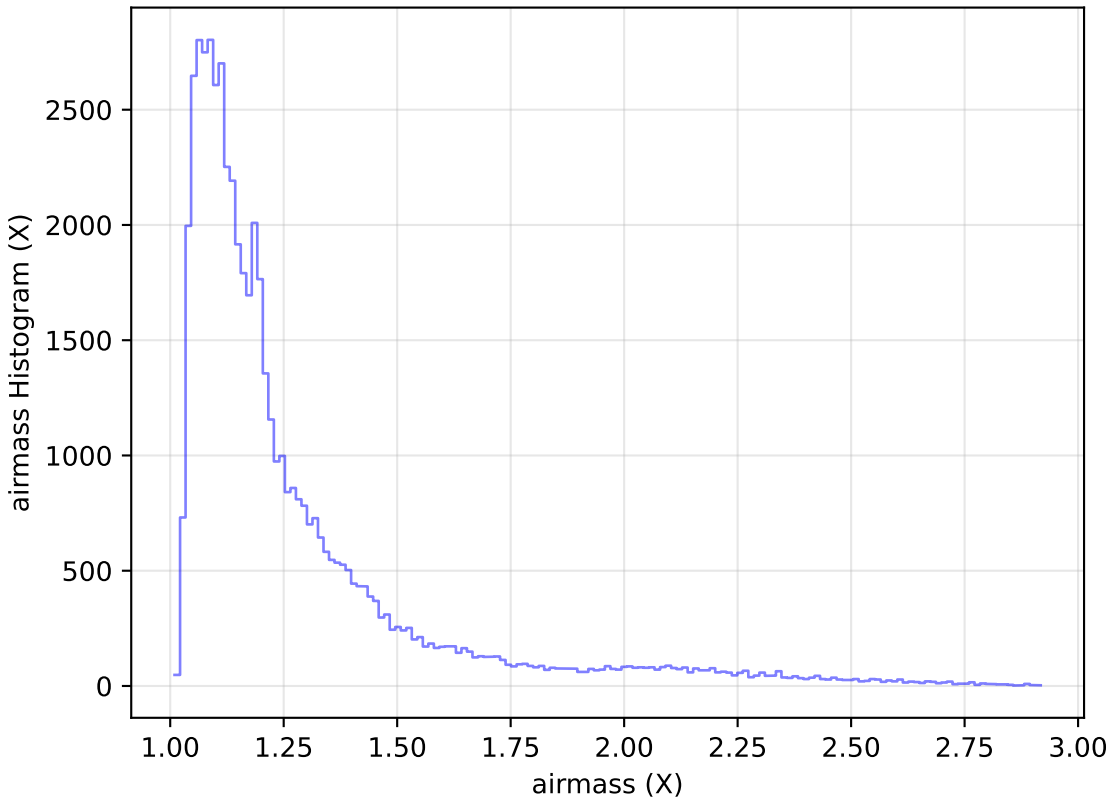
roll_pause_mjdp60_v3.4_10yrs Yr 1 i band: airmass Histogram
