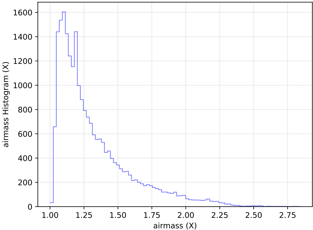
roll_pause_mjdp60_v3.4_10yrs Yr 1 g band: airmass Histogram
