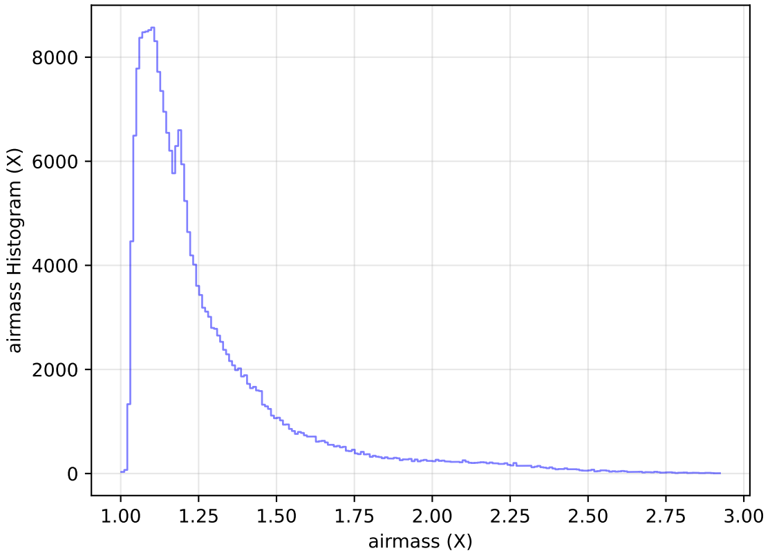
roll_pause_mjdp60_v3.4_10yrs Yr 1 all bands: airmass Histogram
