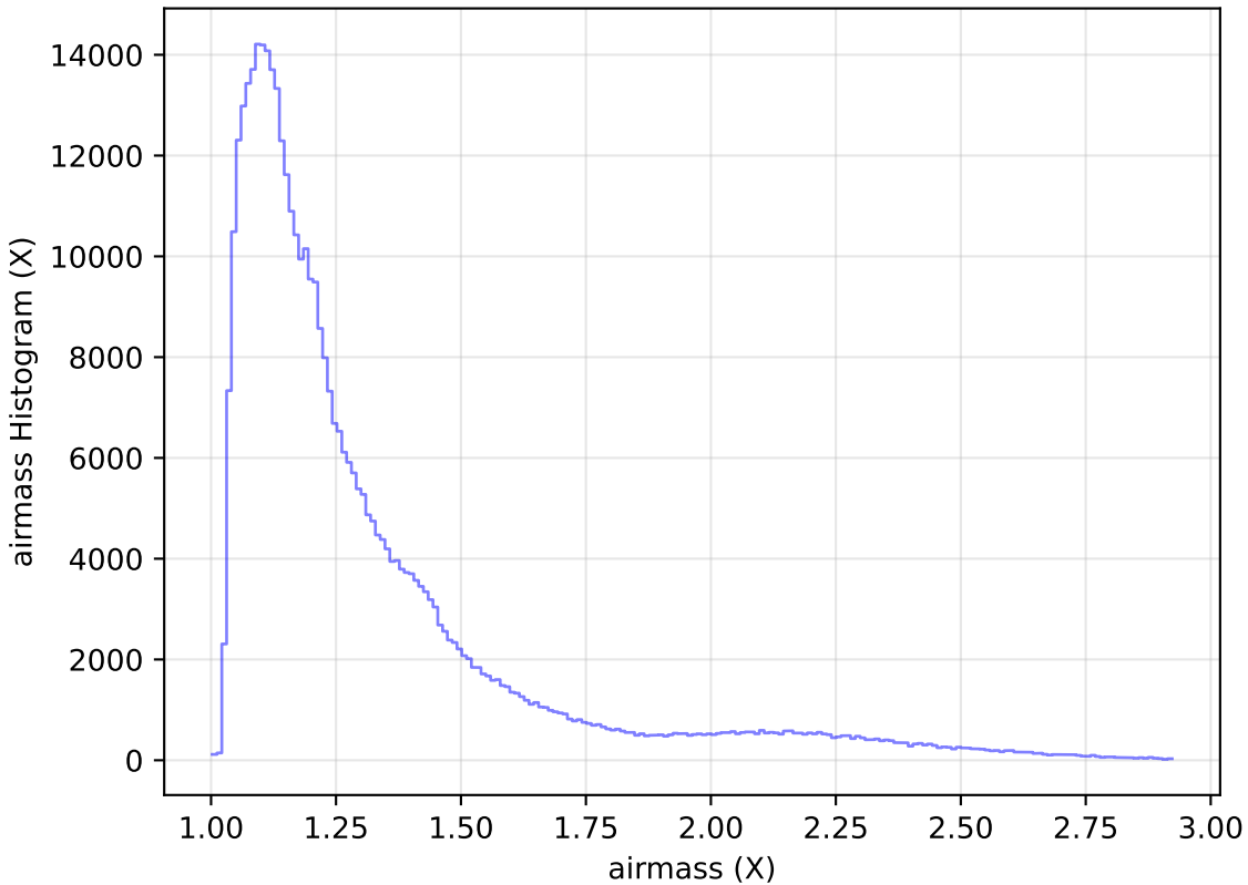
roll_pause_mjdp60_v3.4_10yrs WFD z band: airmass Histogram
