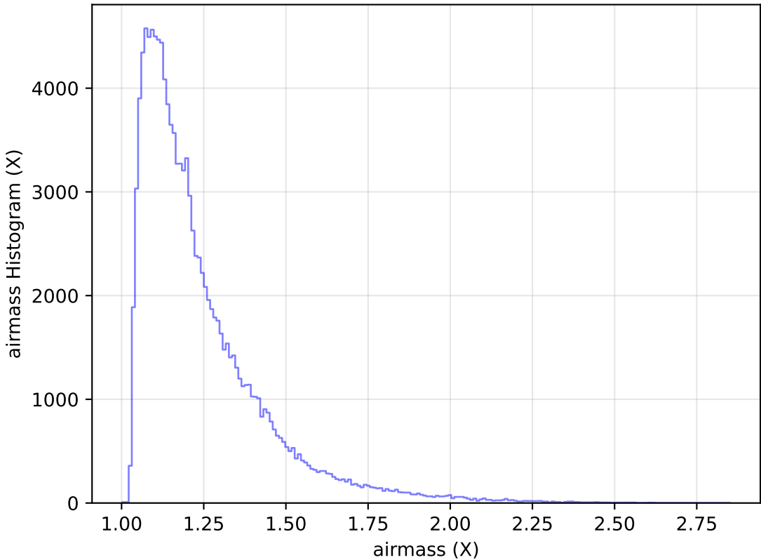
roll_pause_mjdp60_v3.4_10yrs WFD u band: airmass Histogram
