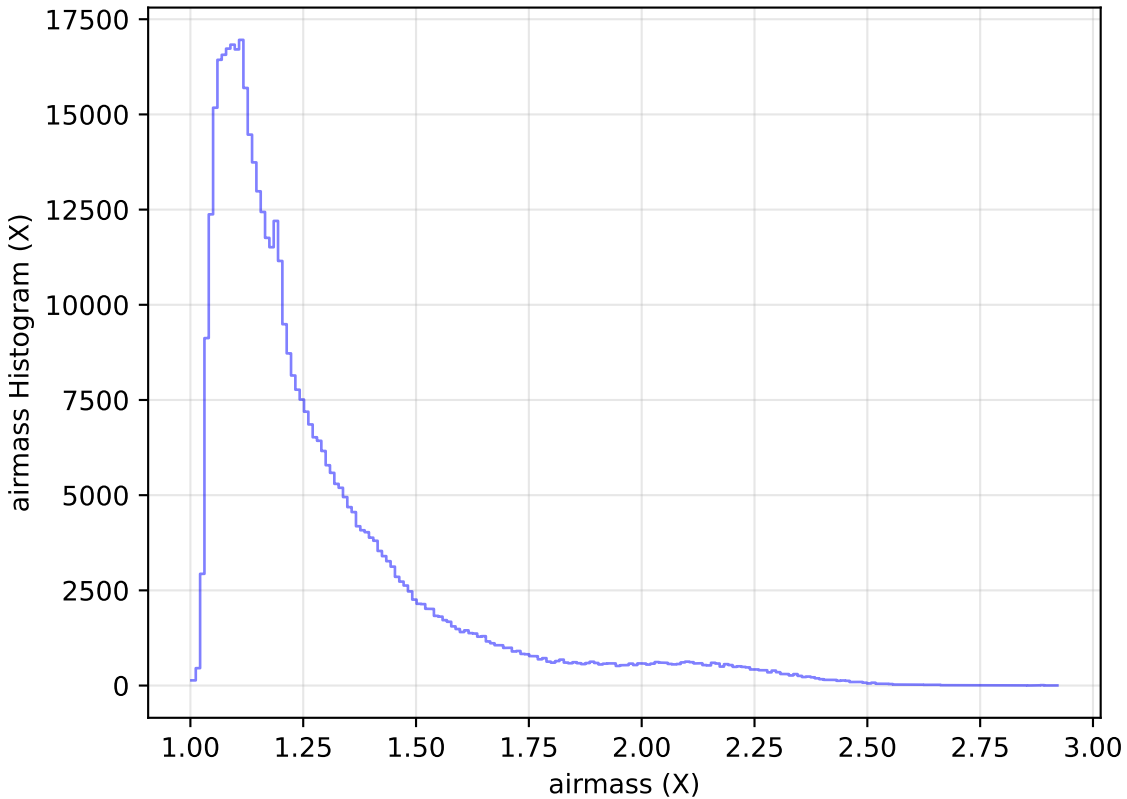
roll_pause_mjdp60_v3.4_10yrs WFD r band: airmass Histogram
