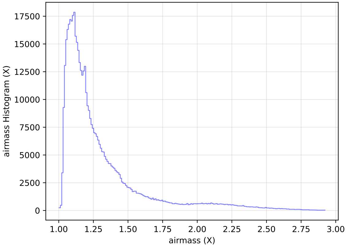
roll_pause_mjdp60_v3.4_10yrs WFD i band: airmass Histogram
