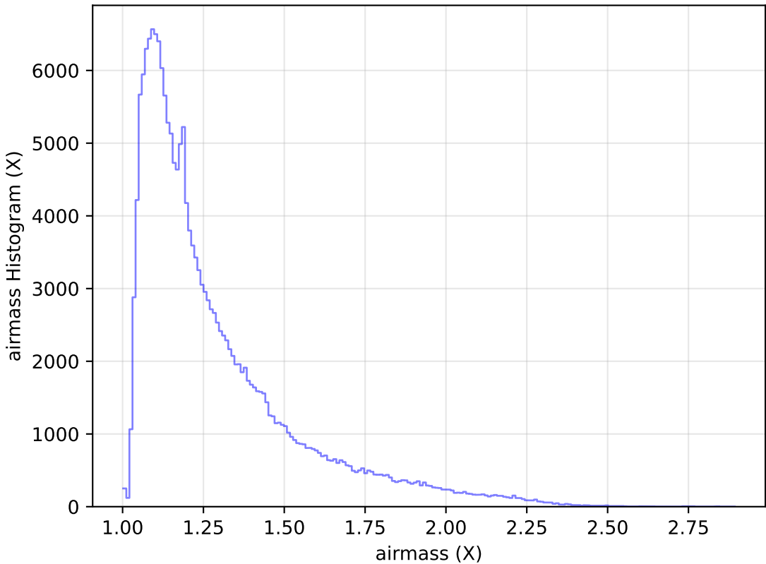
roll_pause_mjdp60_v3.4_10yrs WFD g band: airmass Histogram
