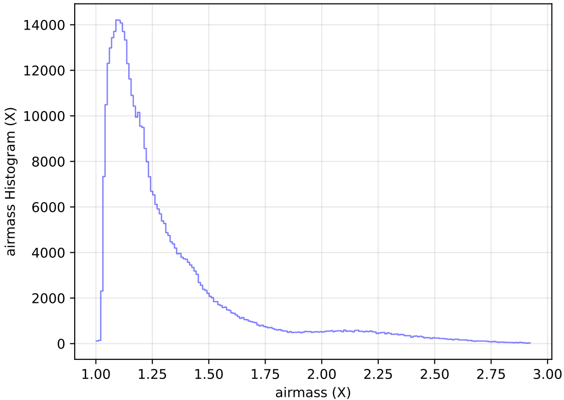
roll_pause_mjdp60_v3.4_10yrs All sky z band: airmass Histogram
