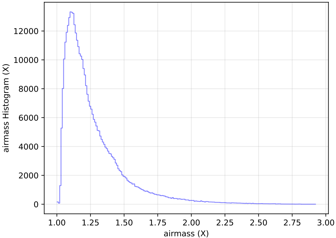
roll_pause_mjdp60_v3.4_10yrs All sky y band: airmass Histogram
